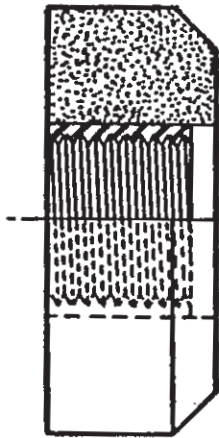
Flange of Insert at Small End of Grinding Wheel as Shown
